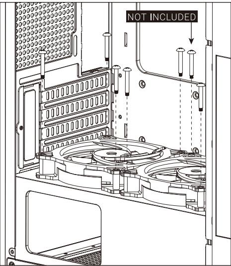
(6d) Install PSU Fans x2
