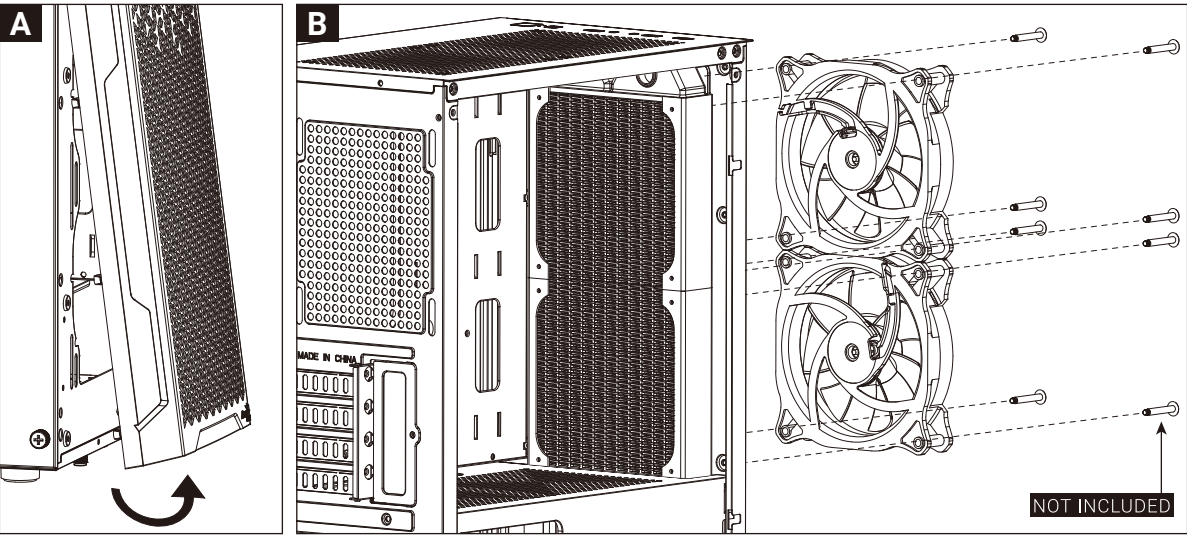
(7a) Install Front Radiator
