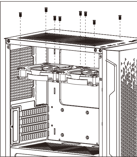
(6b) Install Top Fans x2
