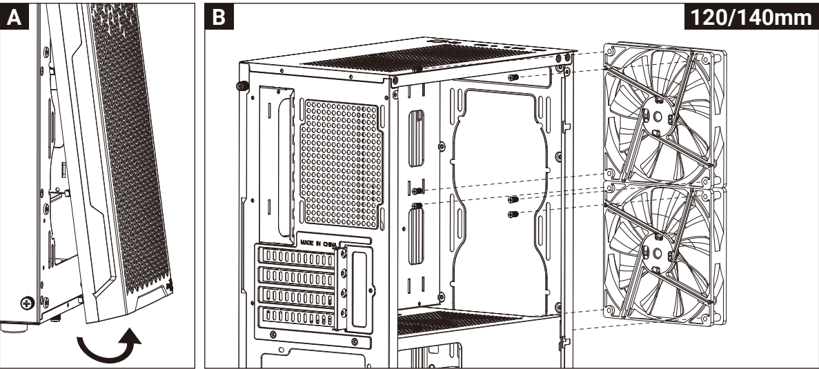
(6a) Install Front Fans
