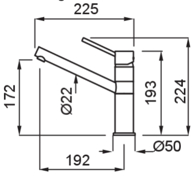
Technical Drawing
