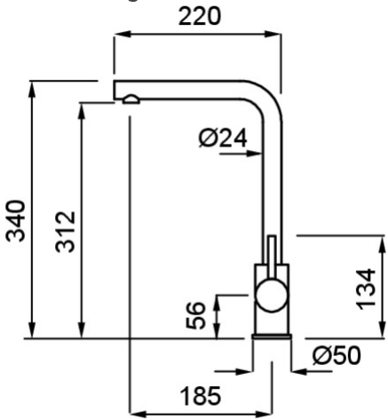
Technical Drawing
