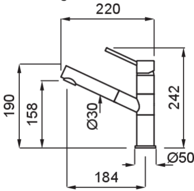
Technical Drawing
