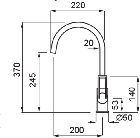
Technical Drawing
