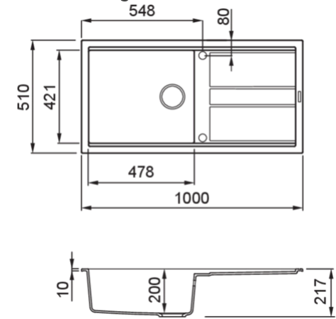
Technical Drawing
